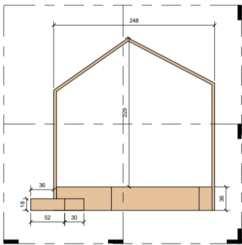
Elevation Left ⑤ 1 : 25
